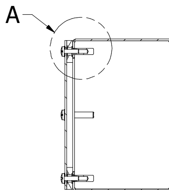
DETAIL A (4 PL.) (LID INSTALL DETAIL)
