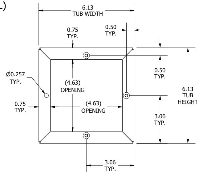
FRONT VIEW (LID AND (1) RIVNUT REMOVED)
