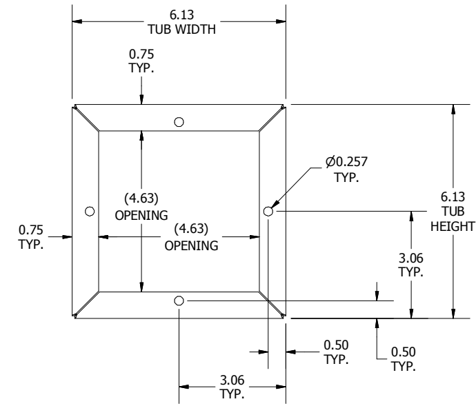
FRONT VIEW, TUB ONLY
