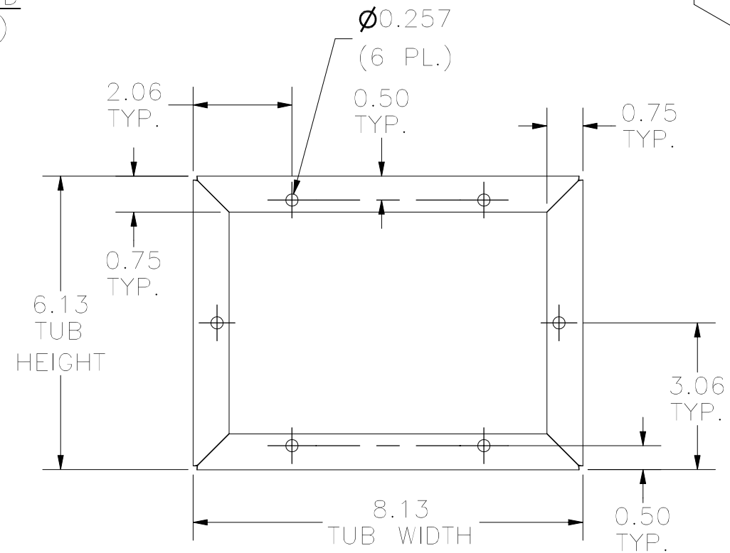
FRONT VIEW TUB
