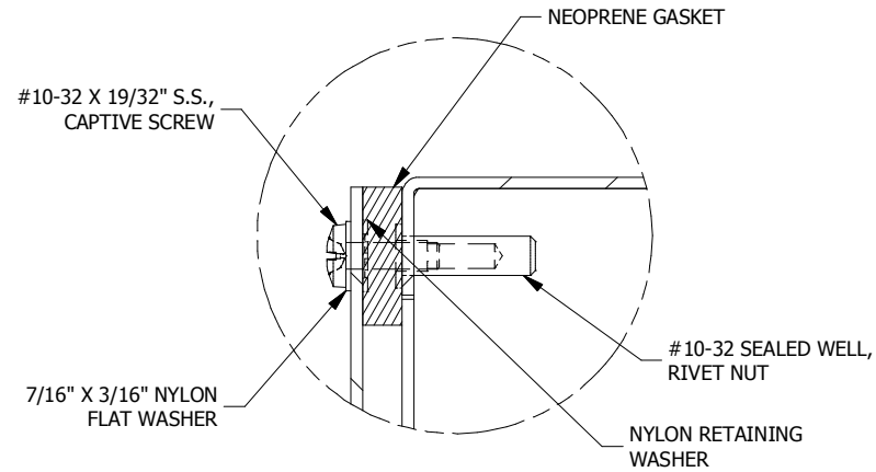
DETAIL A (6 PL.) (LID INSTALL DETAIL)
