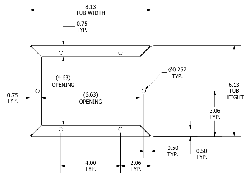
FRONT VIEW, TUB ONLY
