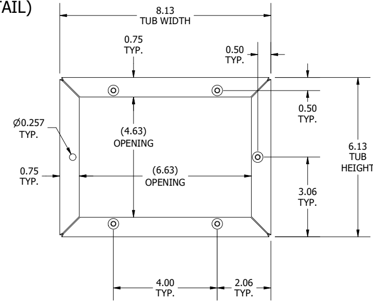
FRONT VIEW (LID AND (1) RIVNUT REMOVED)
