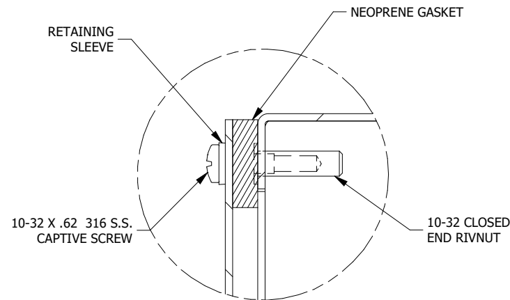
DETAIL A (4 PL.) (LID INSTALL DETAIL)
