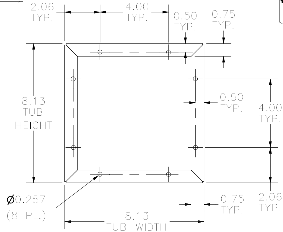
FRONT VIEW TUB
