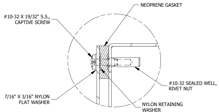
DETAIL A (8 PL.) (LID INSTALL DETAIL)
