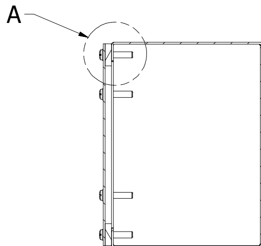
DETAIL A (8 PL.) (LID INSTALL DETAIL)
