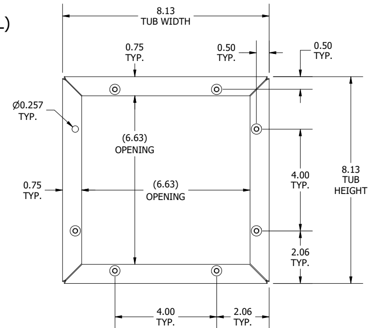
FRONT VIEW (LID AND (1) RIVNUT REMOVED)
