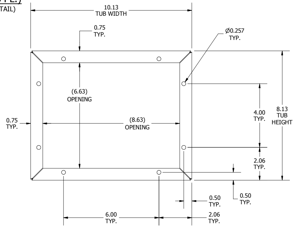
FRONT VIEW, TUB ONLY
