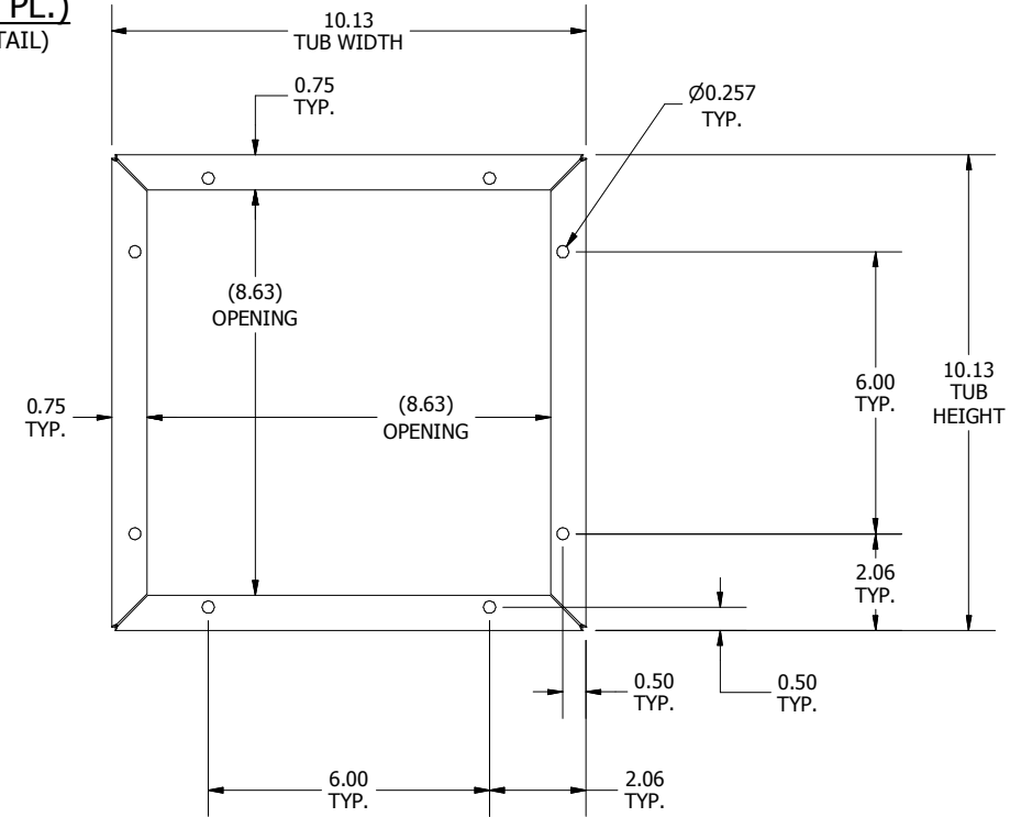
FRONT VIEW, TUB ONLY
