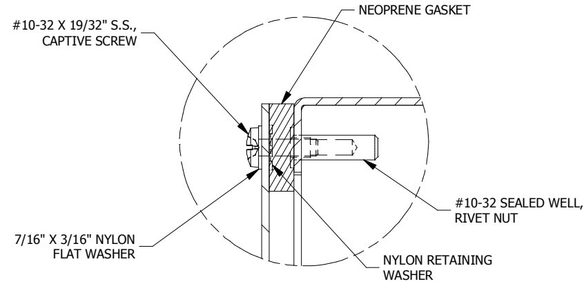
DETAIL A (8 PL.) (LID INSTALL DETAIL)
