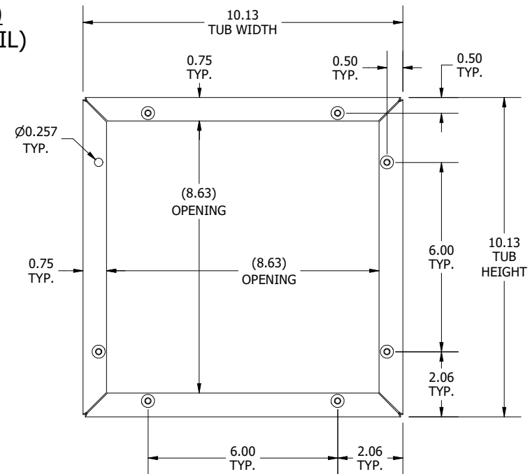
FRONT VIEW (LID AND (1) RIVNUT REMOVED)
