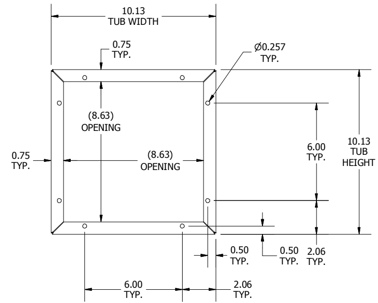
FRONT VIEW, TUB ONLY
