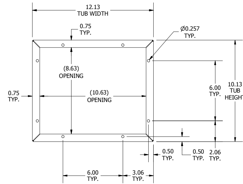
FRONT VIEW, TUB ONLY
