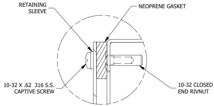
DETAIL A (8 PL.) (LID INSTALL DETAIL)
