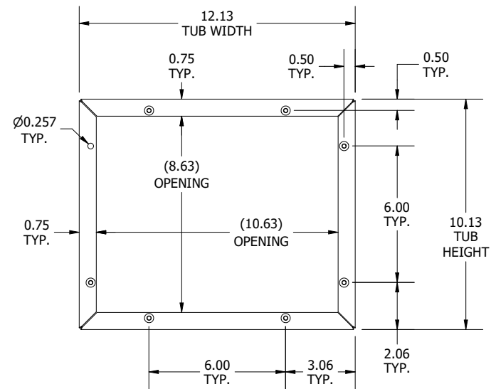
FRONT VIEW (LID AND (1) RIVNUT REMOVED)
