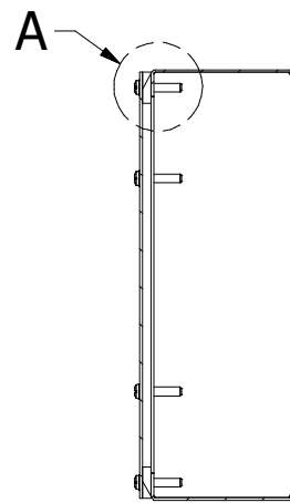
SECTION A-A (INSIDE LEFT OF ENCL.)
