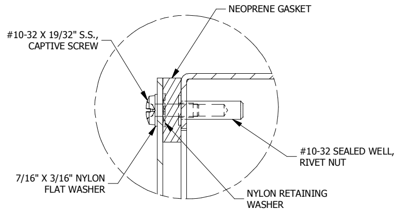
DETAIL A (8 PL.) (LID INSTALL DETAIL)
