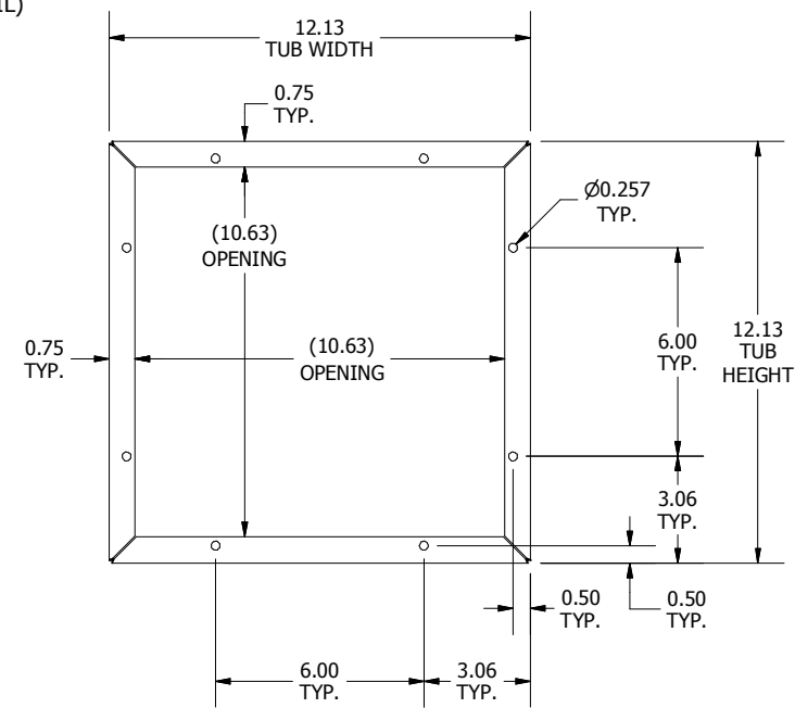
FRONT VIEW, TUB ONLY
