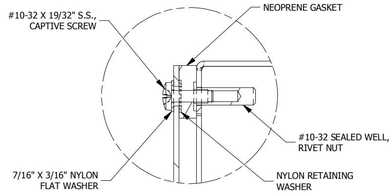
DETAIL A (10 PL.) (LID INSTALL DETAIL)
