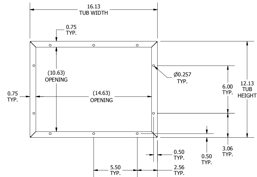
FRONT VIEW, TUB ONLY
