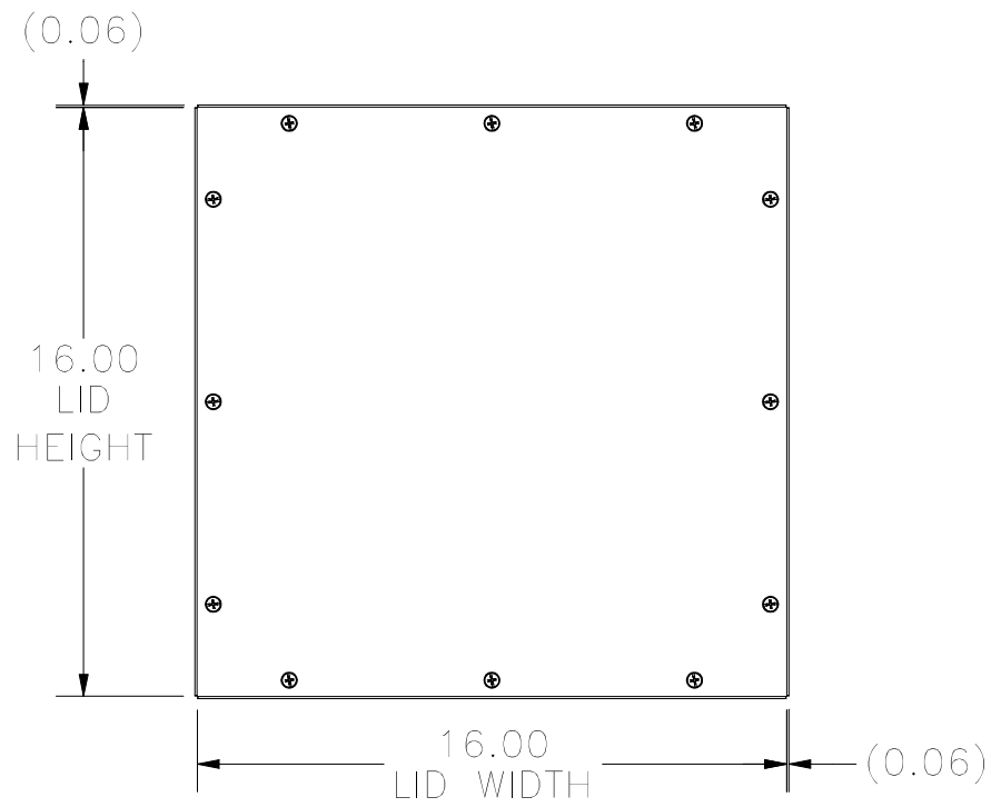
FRONT VIEW
