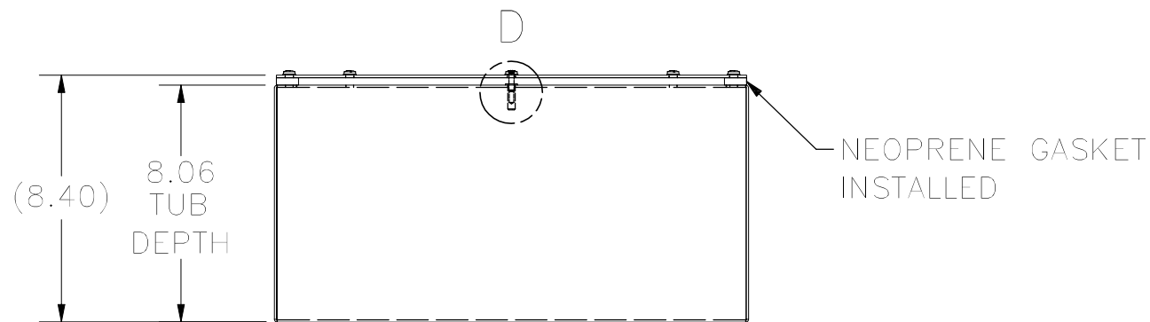
BOTTOM VIEW
