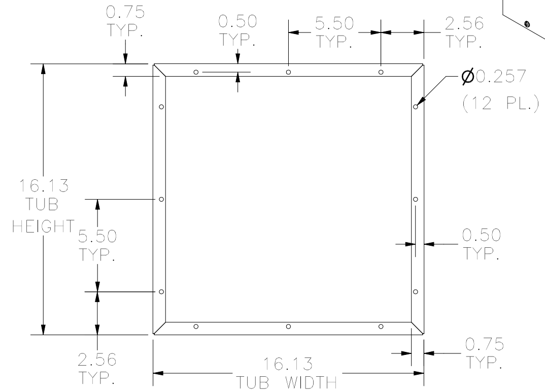
FRONT VIEW TUB
