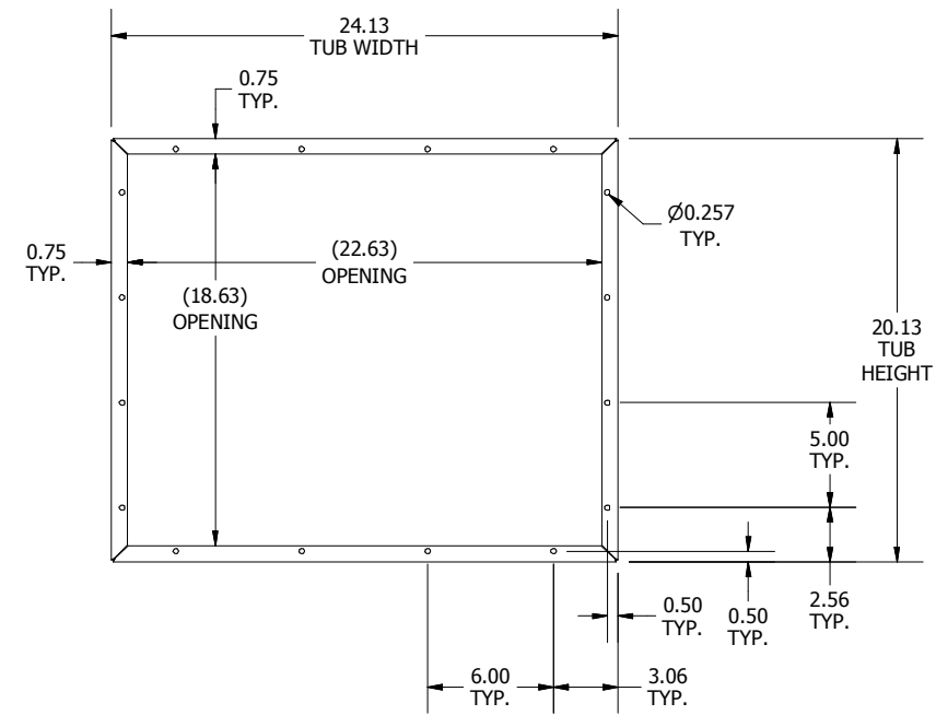
FRONT VIEW, TUB ONLY
