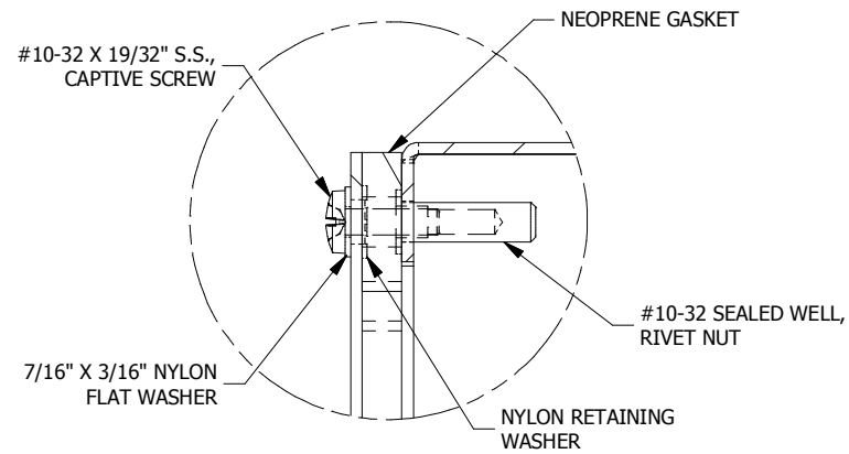
DETAIL A (16 PL.) (LID INSTALL DETAIL)
