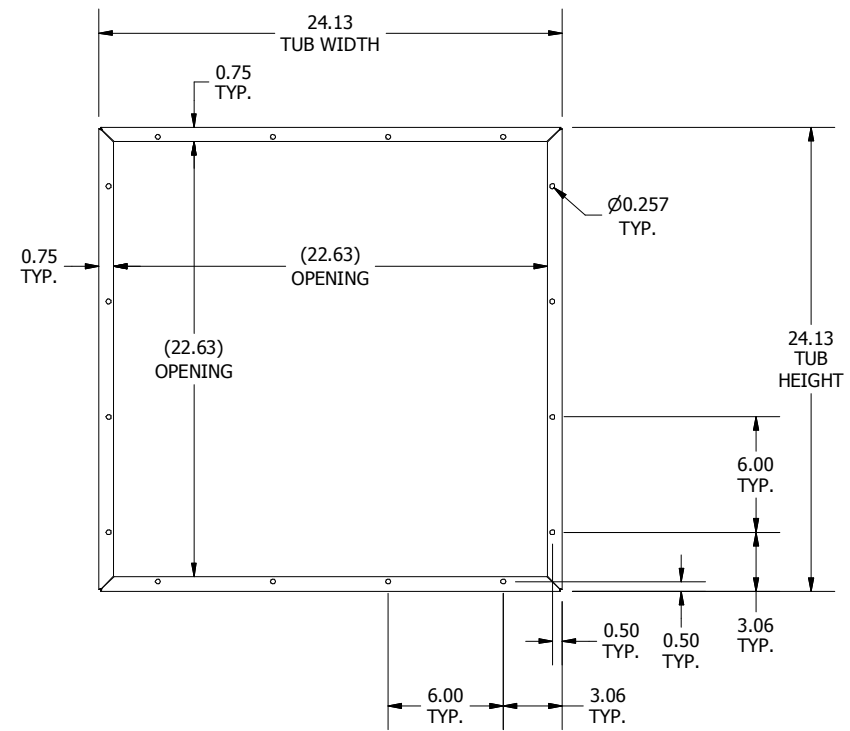
FRONT VIEW, TUB ONLY
