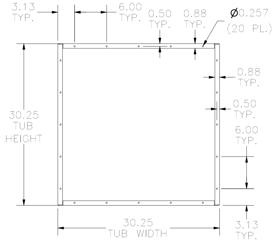
FRONT VIEW TUB
