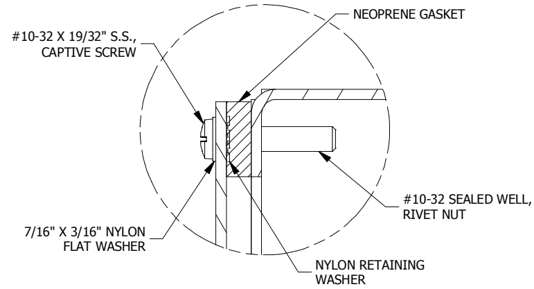
DETAIL A (20 PL.) (LID INSTALL DETAIL)
