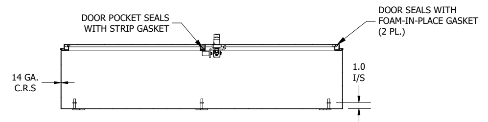
SECTION B-B (INSIDE VIEW OF TOP)
