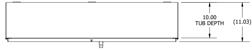
TOP VIEW
