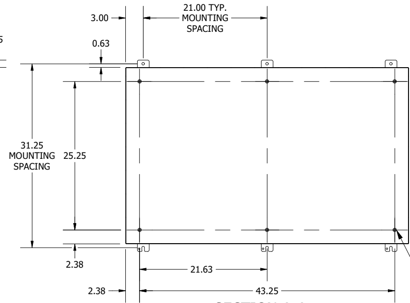
SECTION A-A (INSIDE BACK VIEW OF ENCL.)
