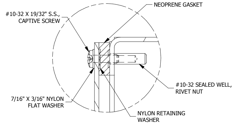
DETAIL A (24 PL.) (LID INSTALL DETAIL)
