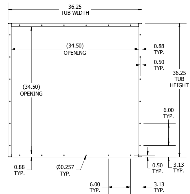
FRONT VIEW, TUB ONLY
