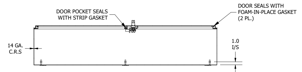
SECTION B-B (INSIDE VIEW OF TOP)
