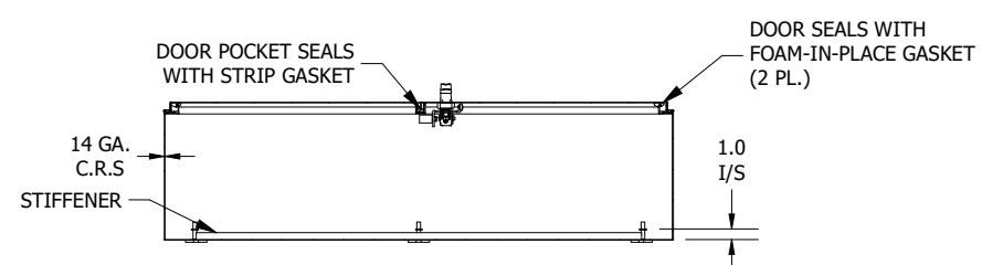
SECTION B-B (INSIDE VIEW OF TOP)
