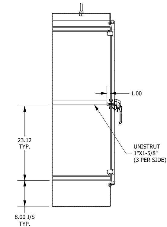
SECTION B-B (INSIDE RIGHT VIEW OF ENCLOSURE)
