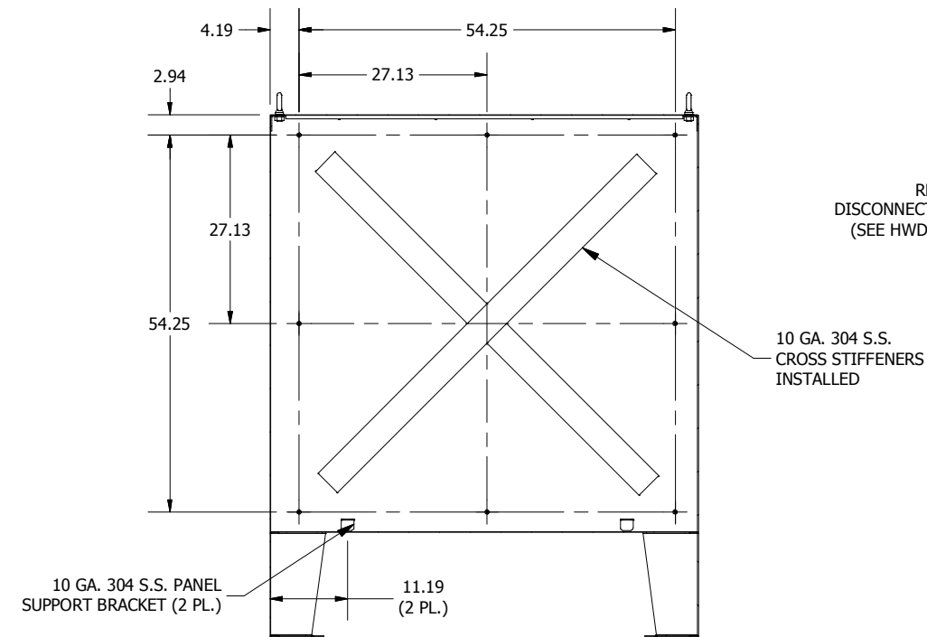
SECTION A-A (INSIDE BACK OF ENCL.)
