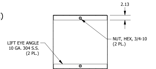
SECTION C-C (INSIDE TOP VIEW OF ENCLOSURE)
