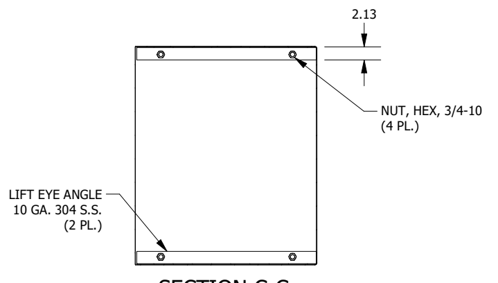
SECTION C-C (INSIDE TOP VIEW OF ENCLOSURE)
