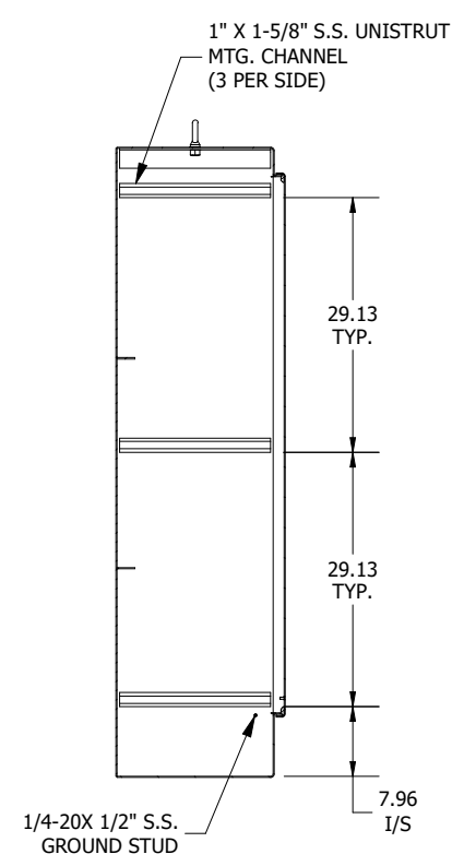
SECTION B-B (INSIDE RIGHT OF ENCL.)
