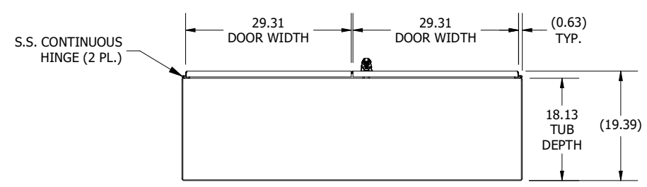
BOTTOM VIEW
