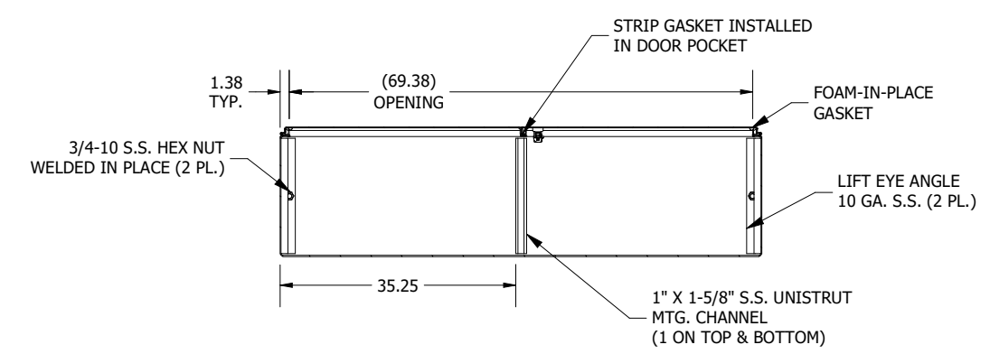
SECTION C-C (INSIDE TOP OF ENCL.)
