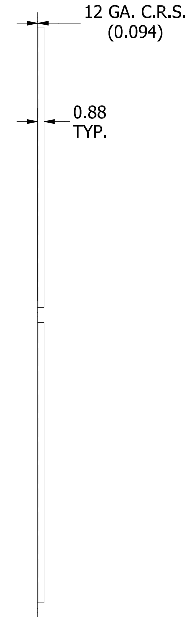
SIDE VIEW
