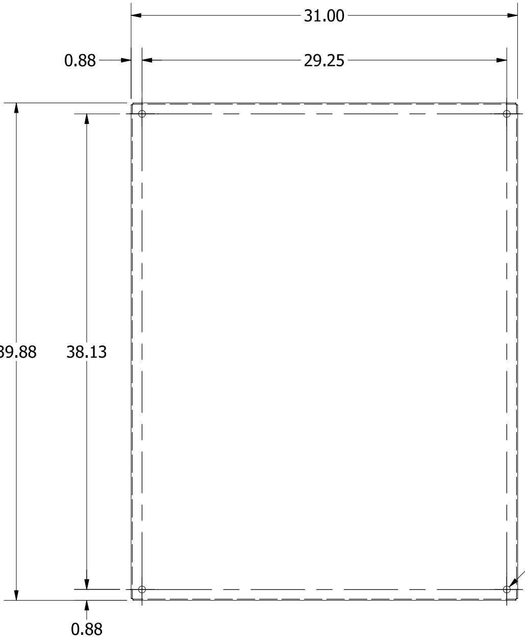
FRONT VIEW
