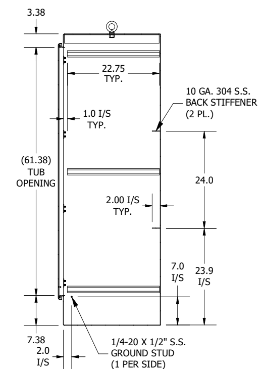
SECTION B-B (INSIDE LEFT OF ENCL.)
