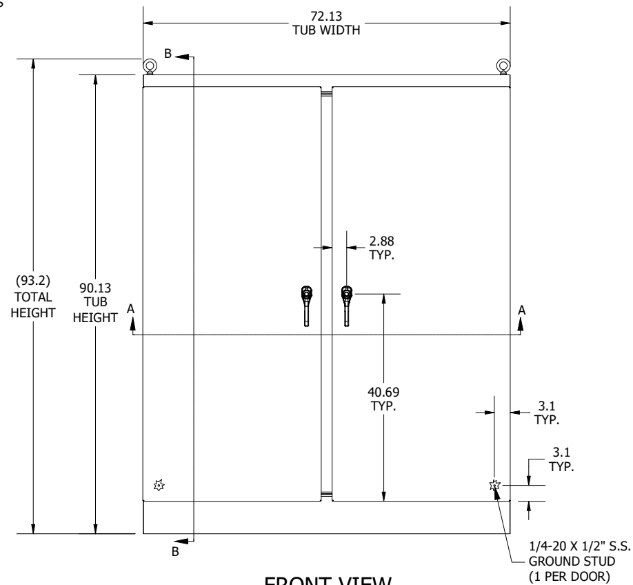
FRONT VIEW
