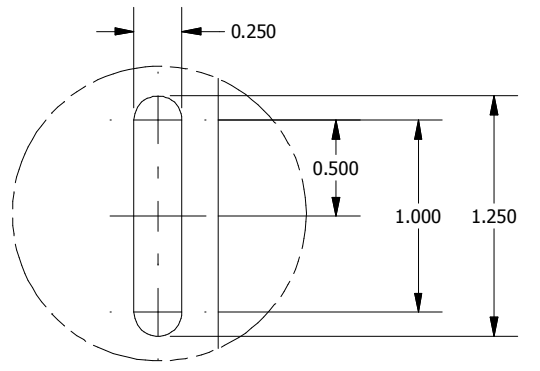
DETAIL A (32 PL.) (SLOT DETAIL)
