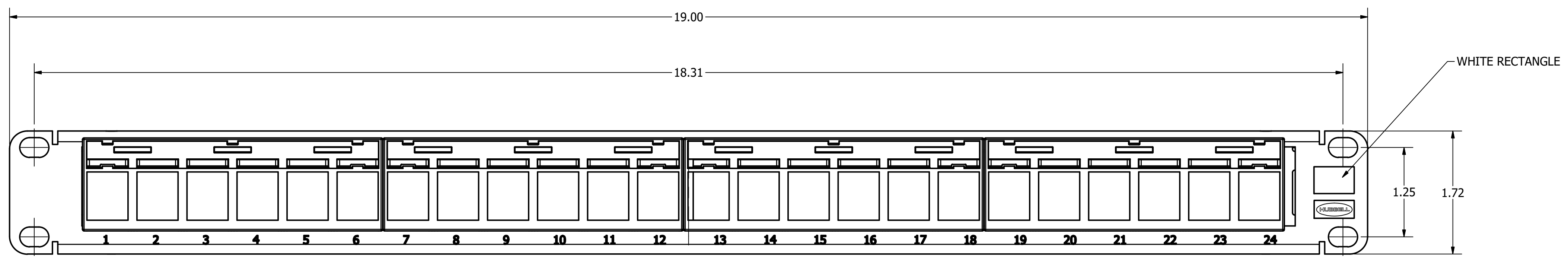
FRONT VIEW
