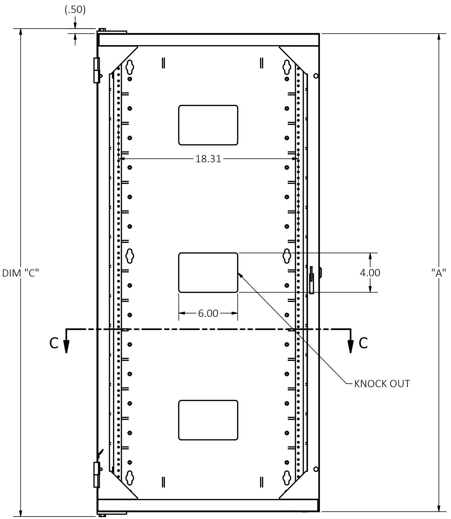
FRONT VIEW (FRONT DOOR NOT SHOWN)
