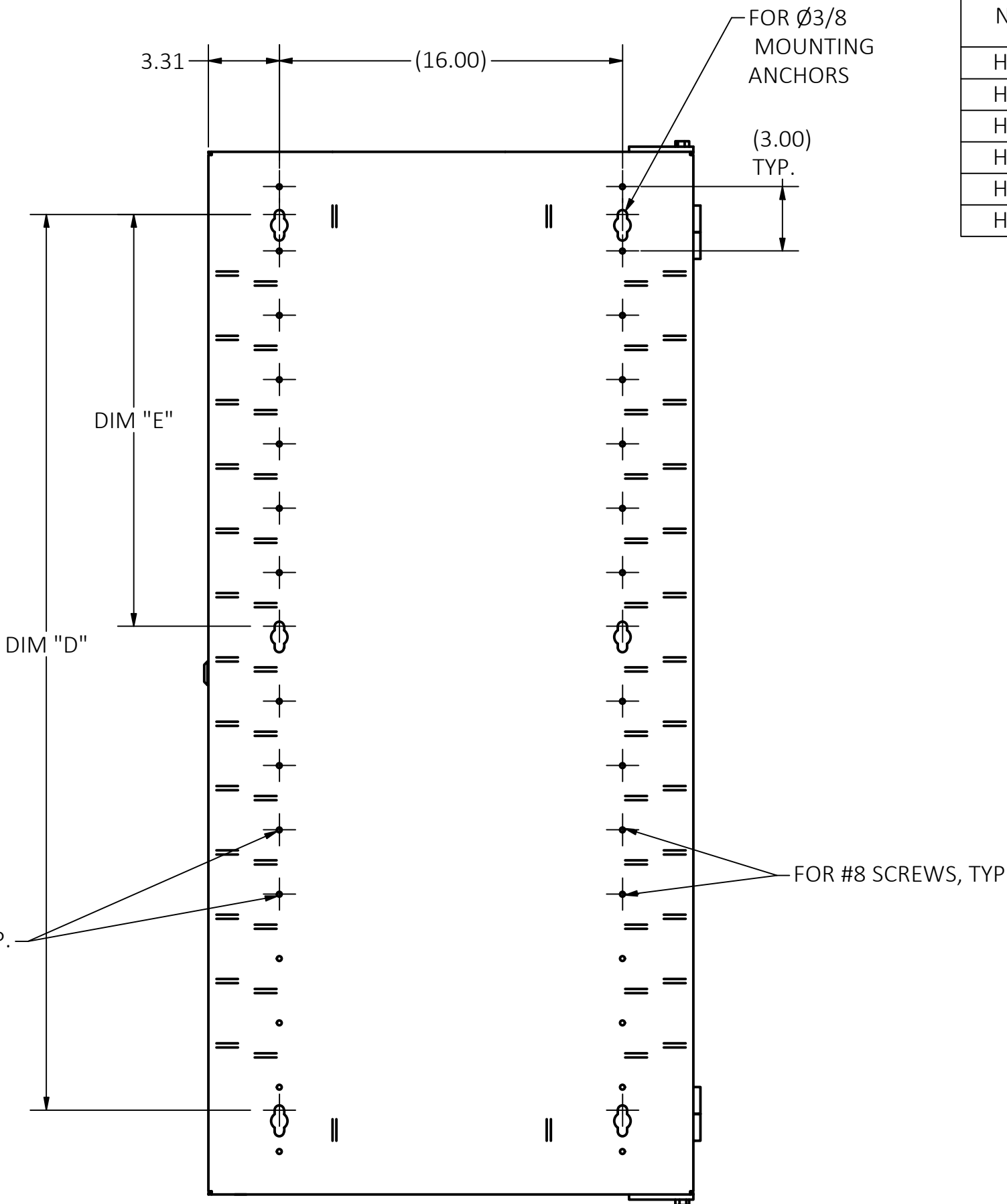
WALL MOUNTING PATTERN
