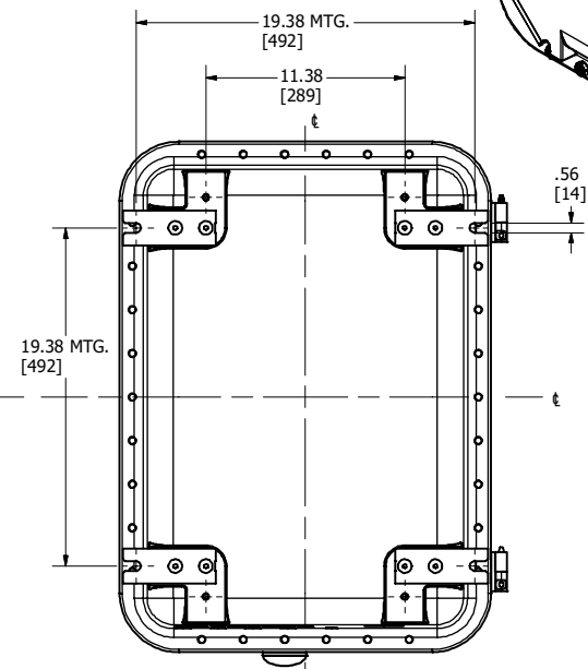
MOUNTING FEET
