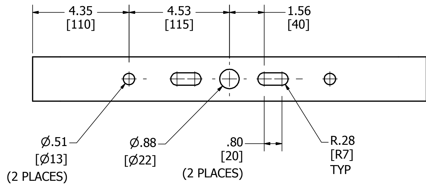
TRUNNION MOUNTING DETAIL
