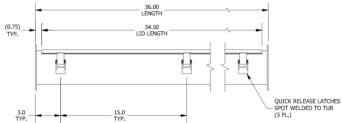
FRONT VIEW
