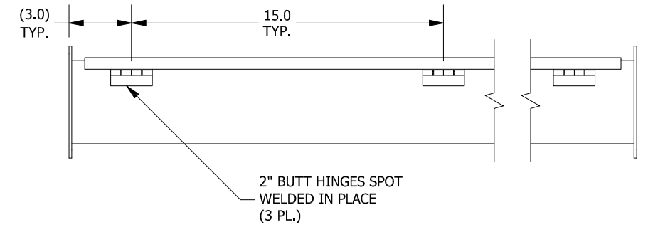
BACK VIEW
