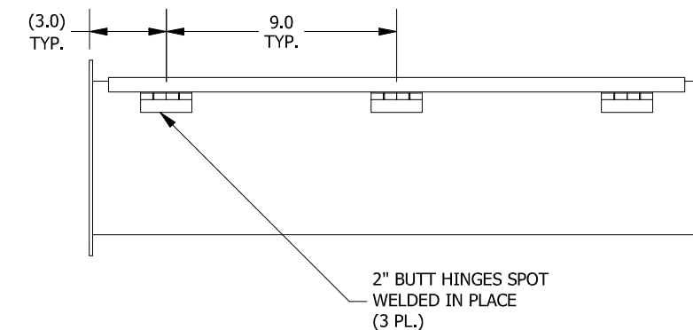
BACK VIEW
