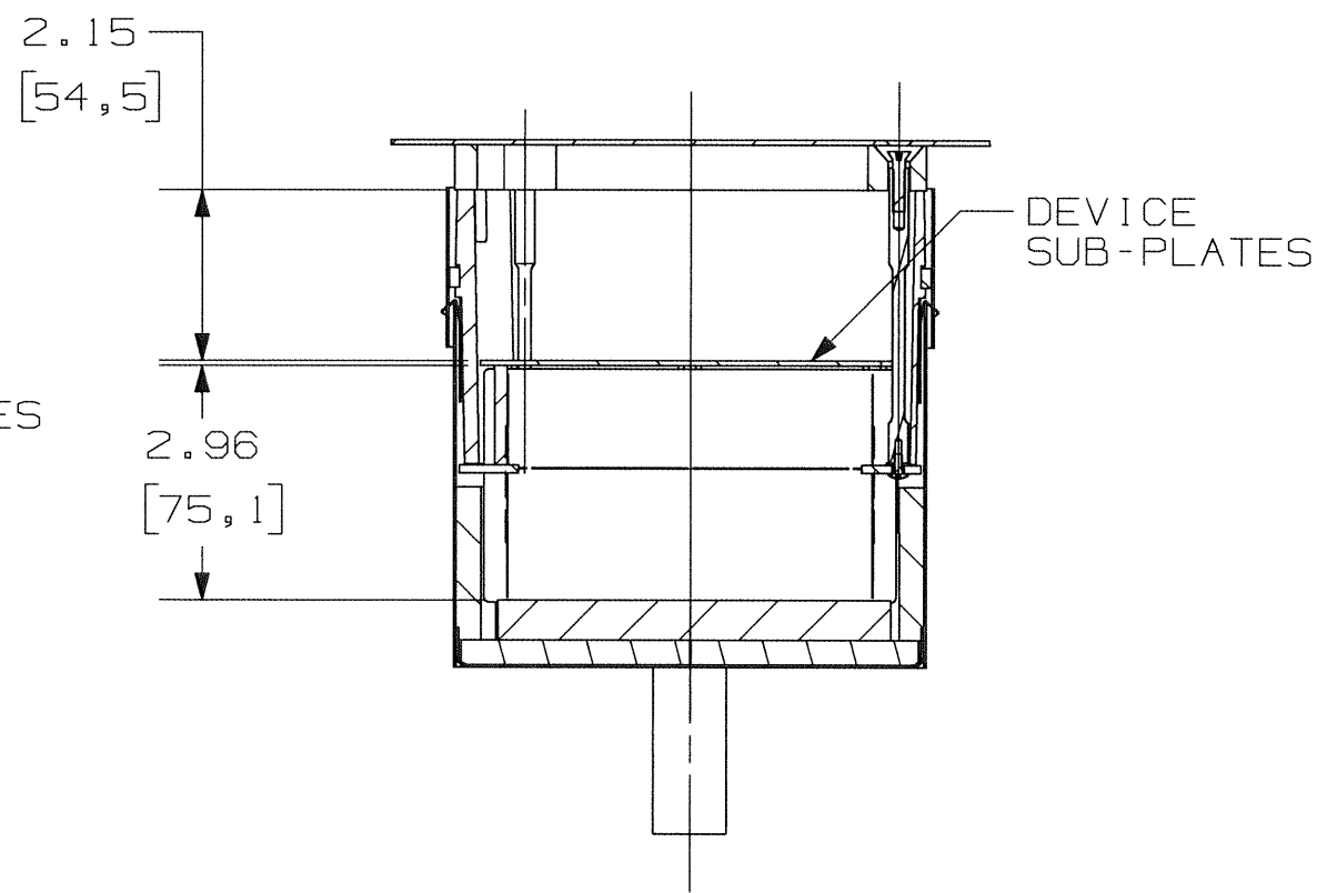
SECTION B-B
