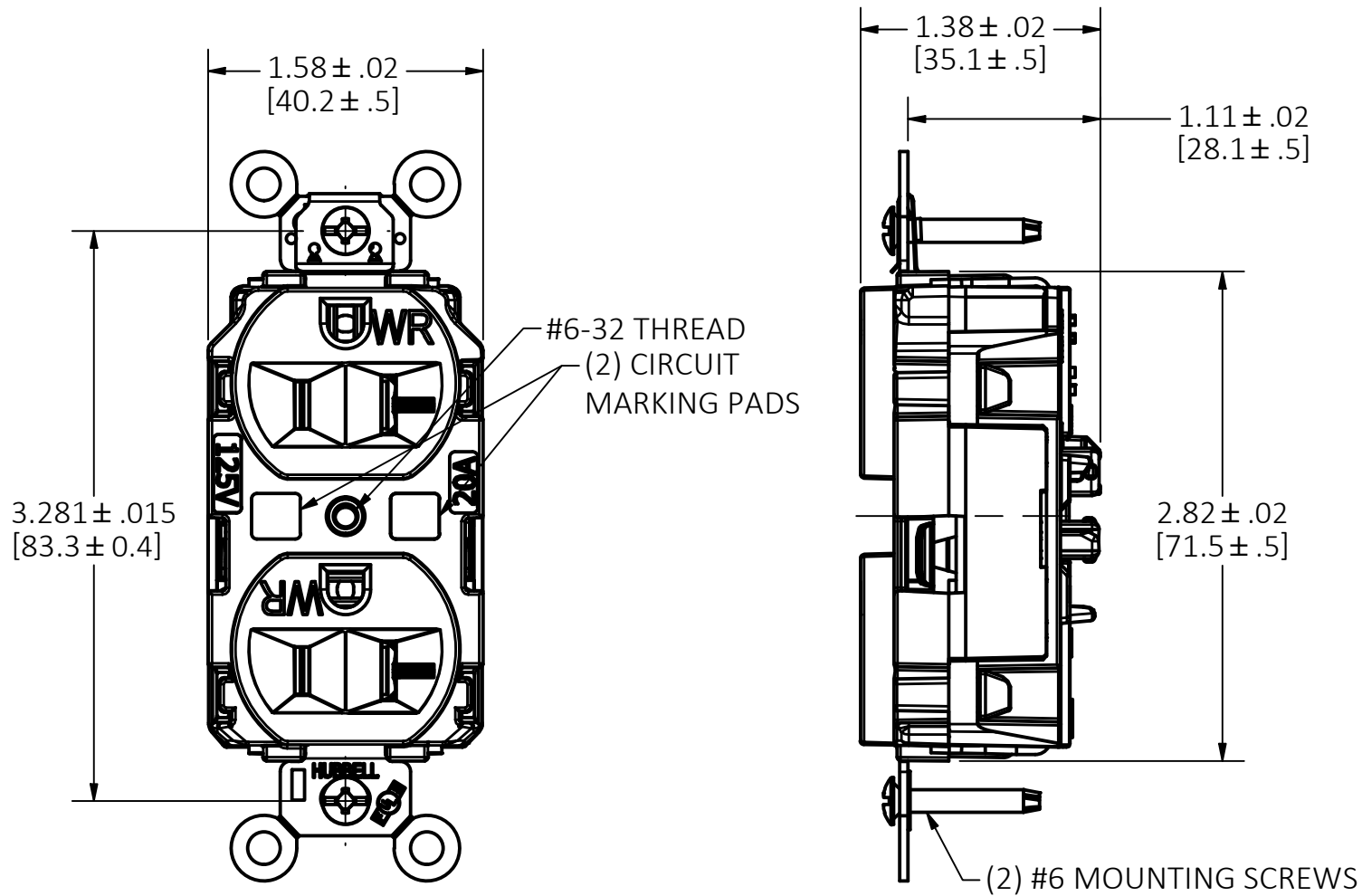
20A/125V DEVICE SHOWN
