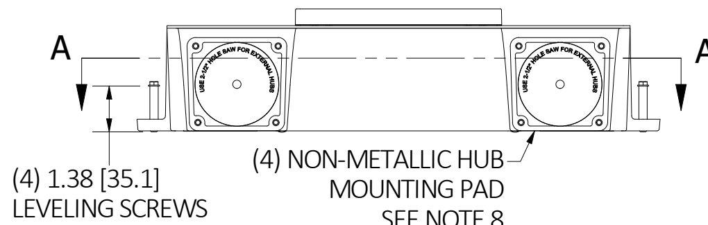
SIDE VIEW
