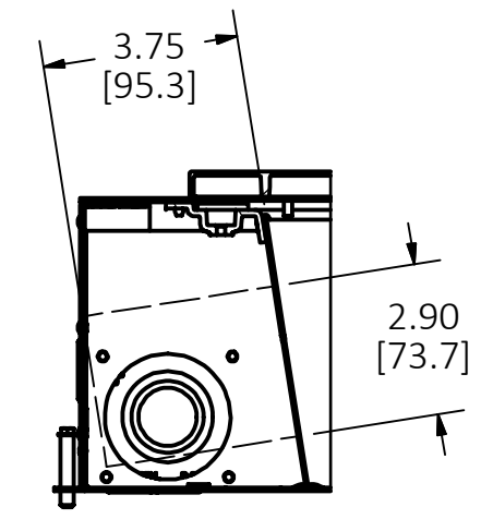
SECTION B-B WIRING CHAMBERS
