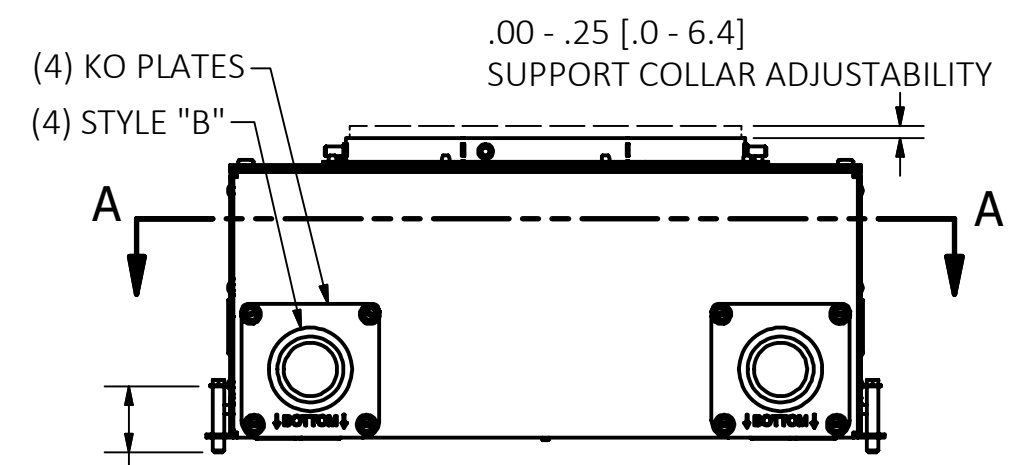
SIDE VIEW TEMP COVER NOT SHOWN
