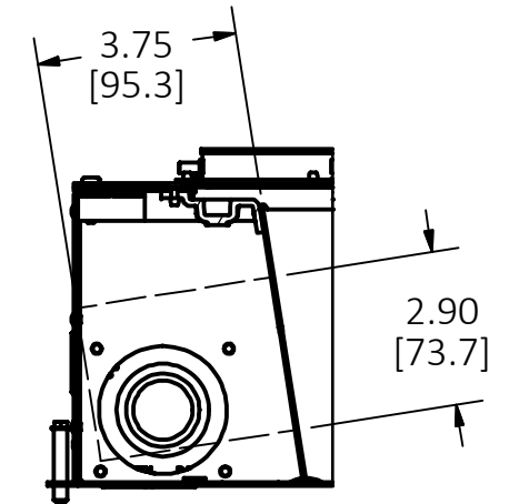
SECTION B-B WIRING CHAMBERS
