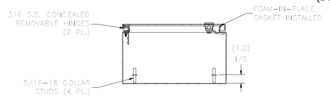
SECTION B-B VIEW (INSIDE TOP OF ENCL.)
